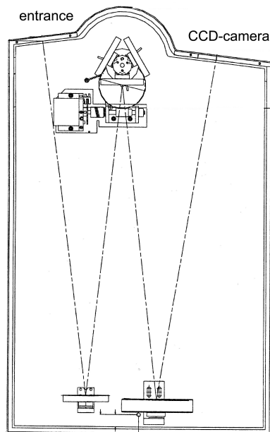
Figure 7: Schematic diagram of the TRIAX 550 spectrometer. The optical path is drawn. In the upper part the adjustable grating that decomposes light in its spectrum is illustrated.
